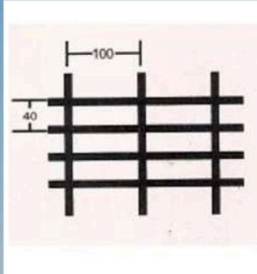
ARC MS- 40x100
