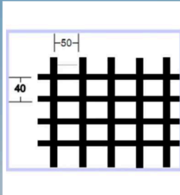
ARC SS - 40x50 Gratings
