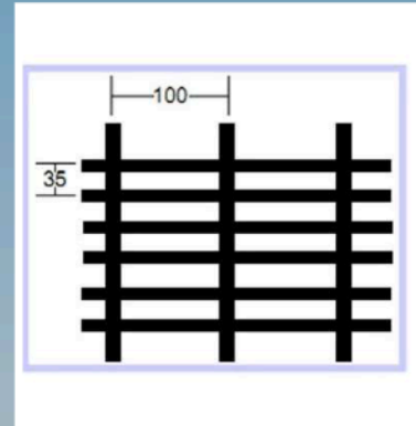
ARC SS - 35x100 Gratings
